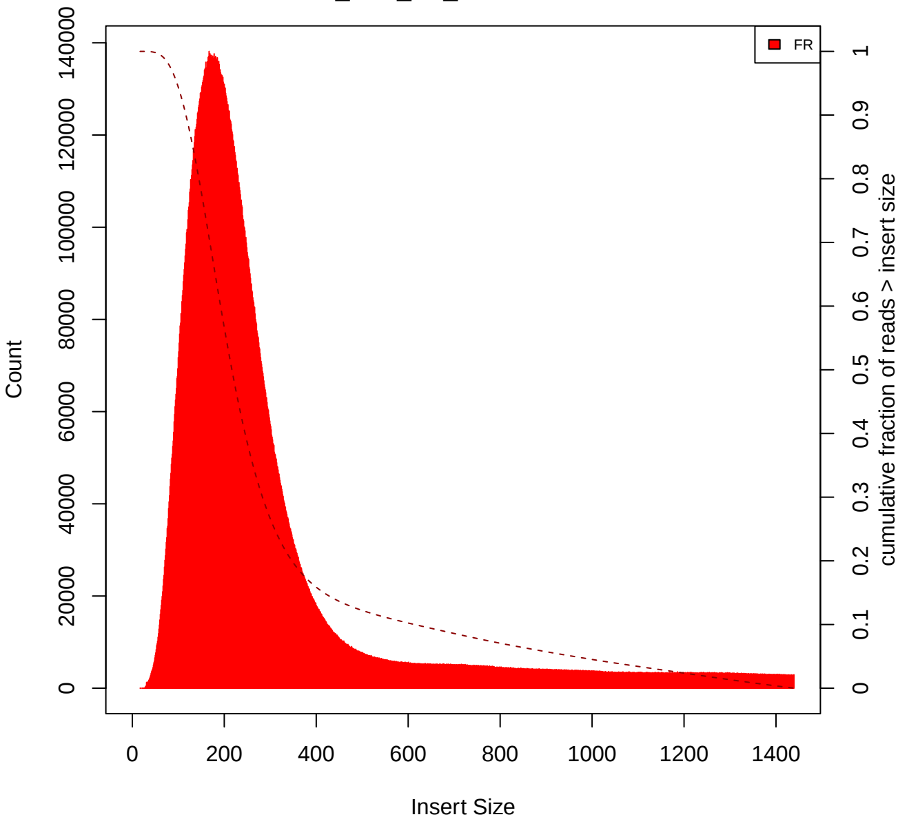
Insert Size Histogram for All_Reads in file GRCh37-HSC_D12_TA_1uM.samtools-coordinate.bam
