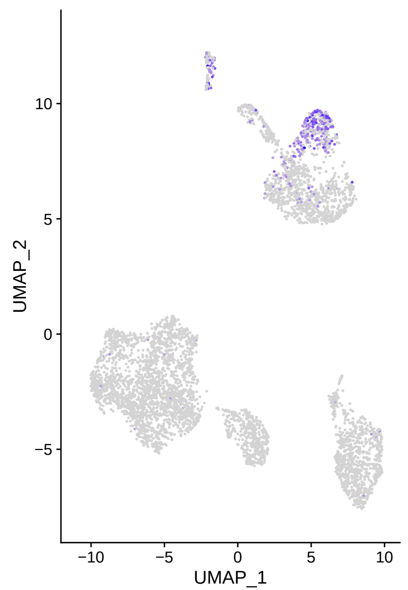
PRTG
