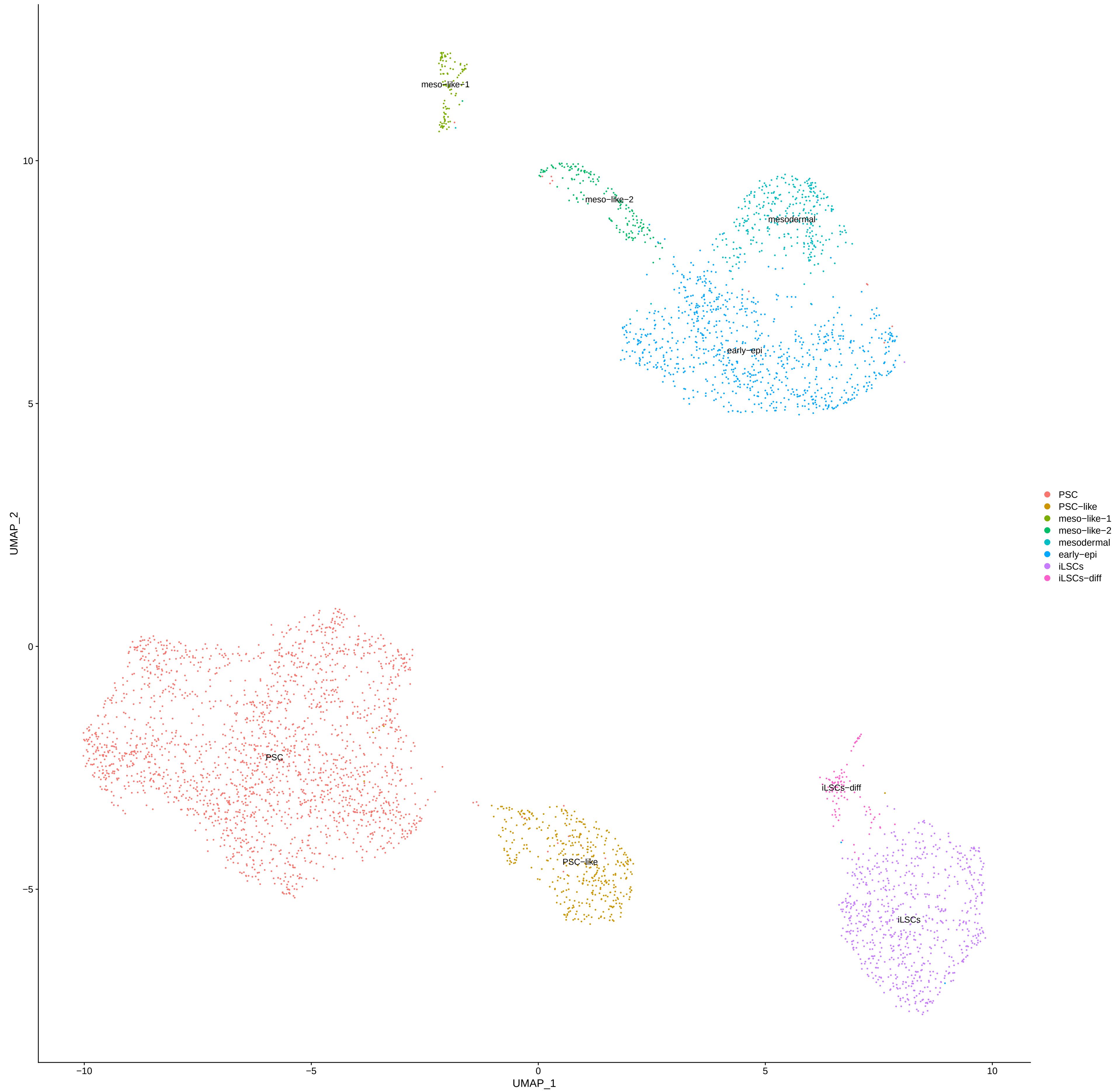
Louvain Clustering
