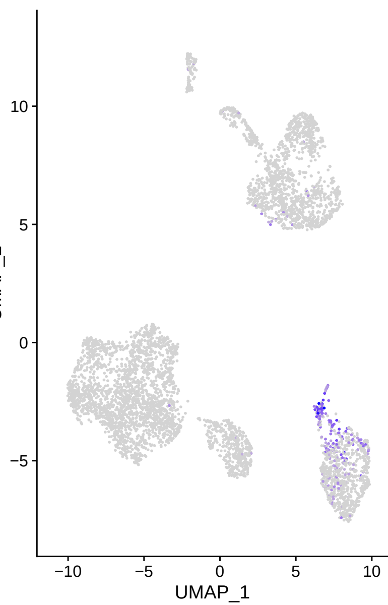
UPK1B
