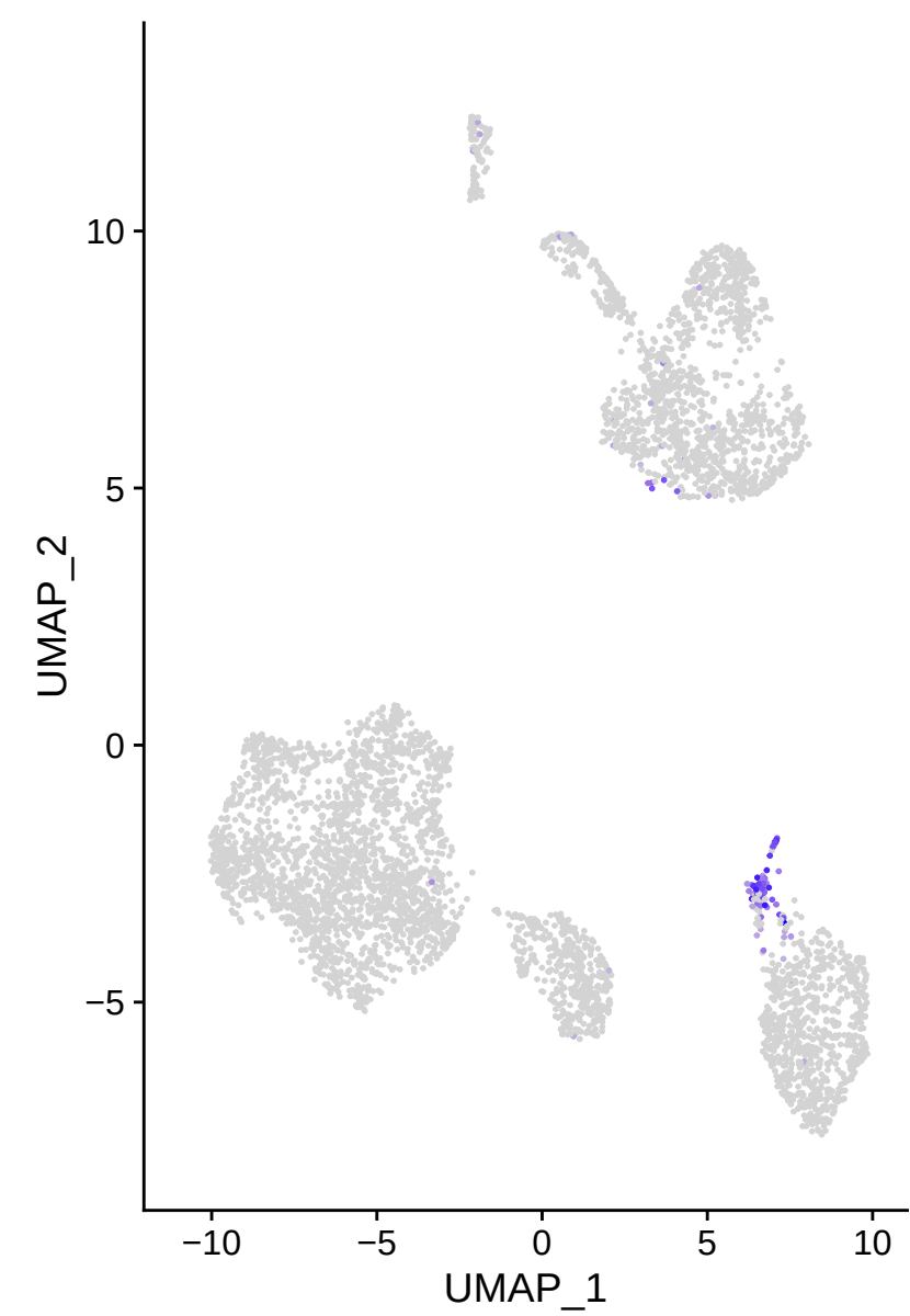
KRT23
