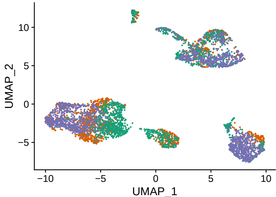
cell_type
