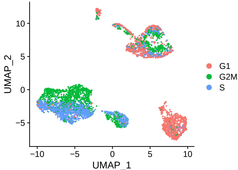
Phase
