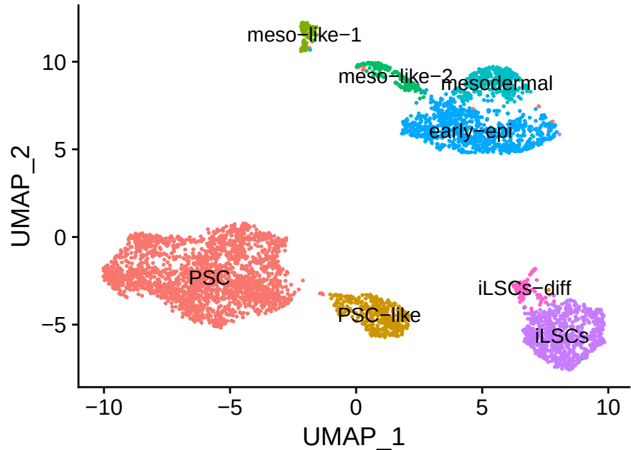
Louvain Clustering
