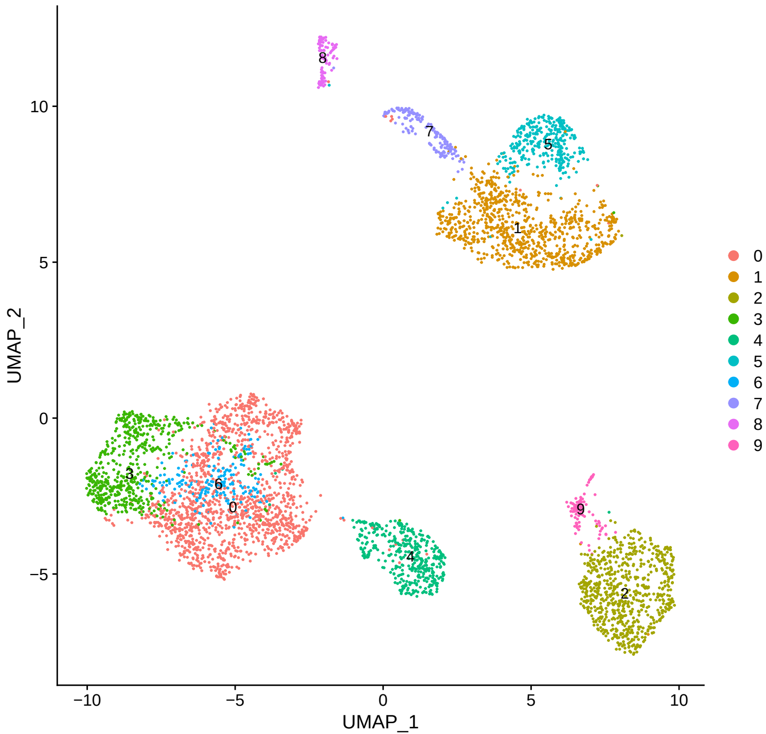
cluster resolution 0.4
