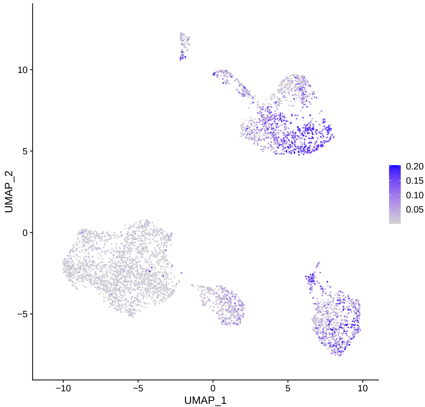
decontX_contamination
