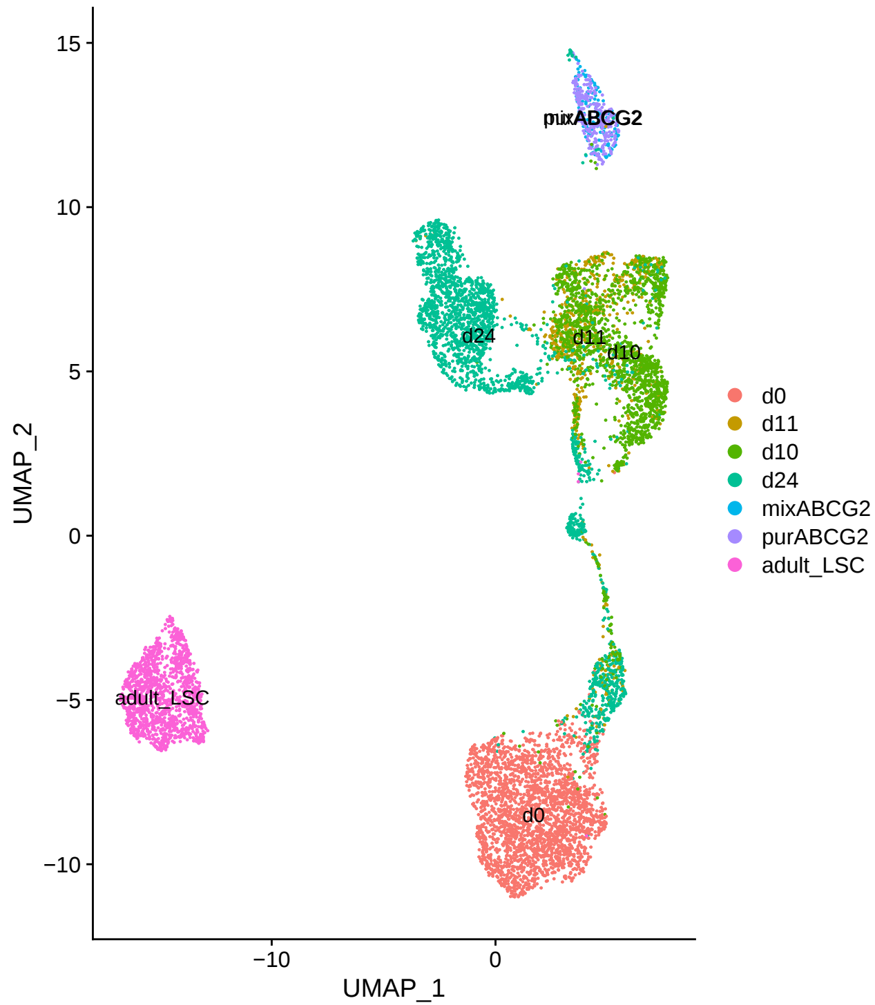
cluster resolution 1.2
