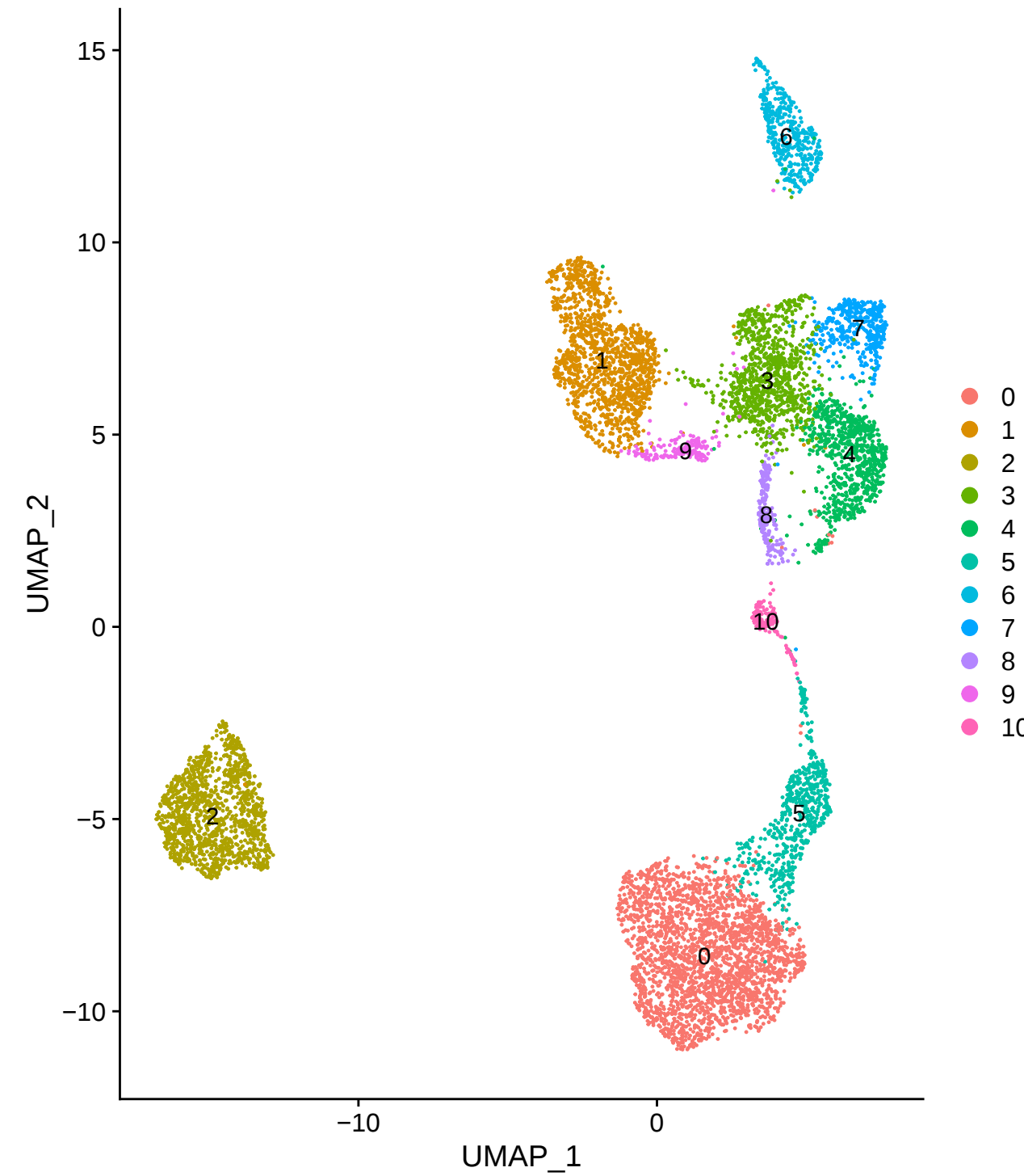
cluster resolution 0.4
