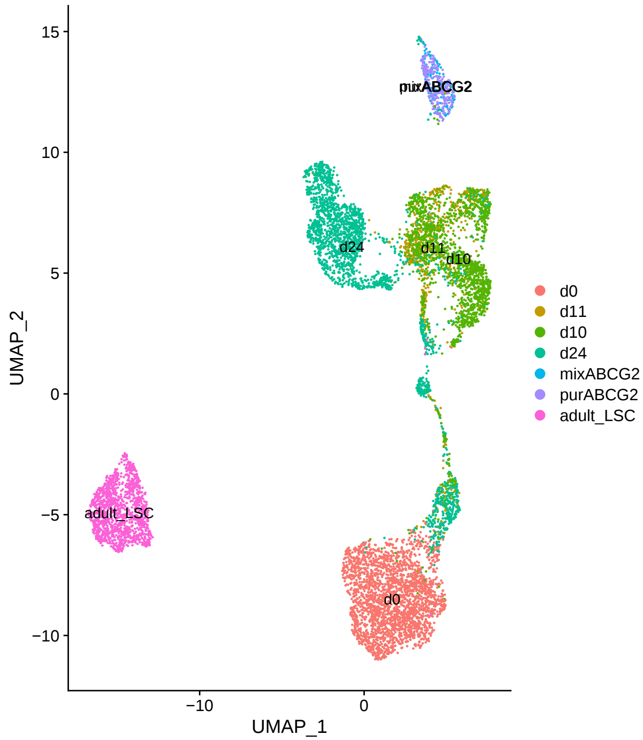
cluster resolution 0.3
