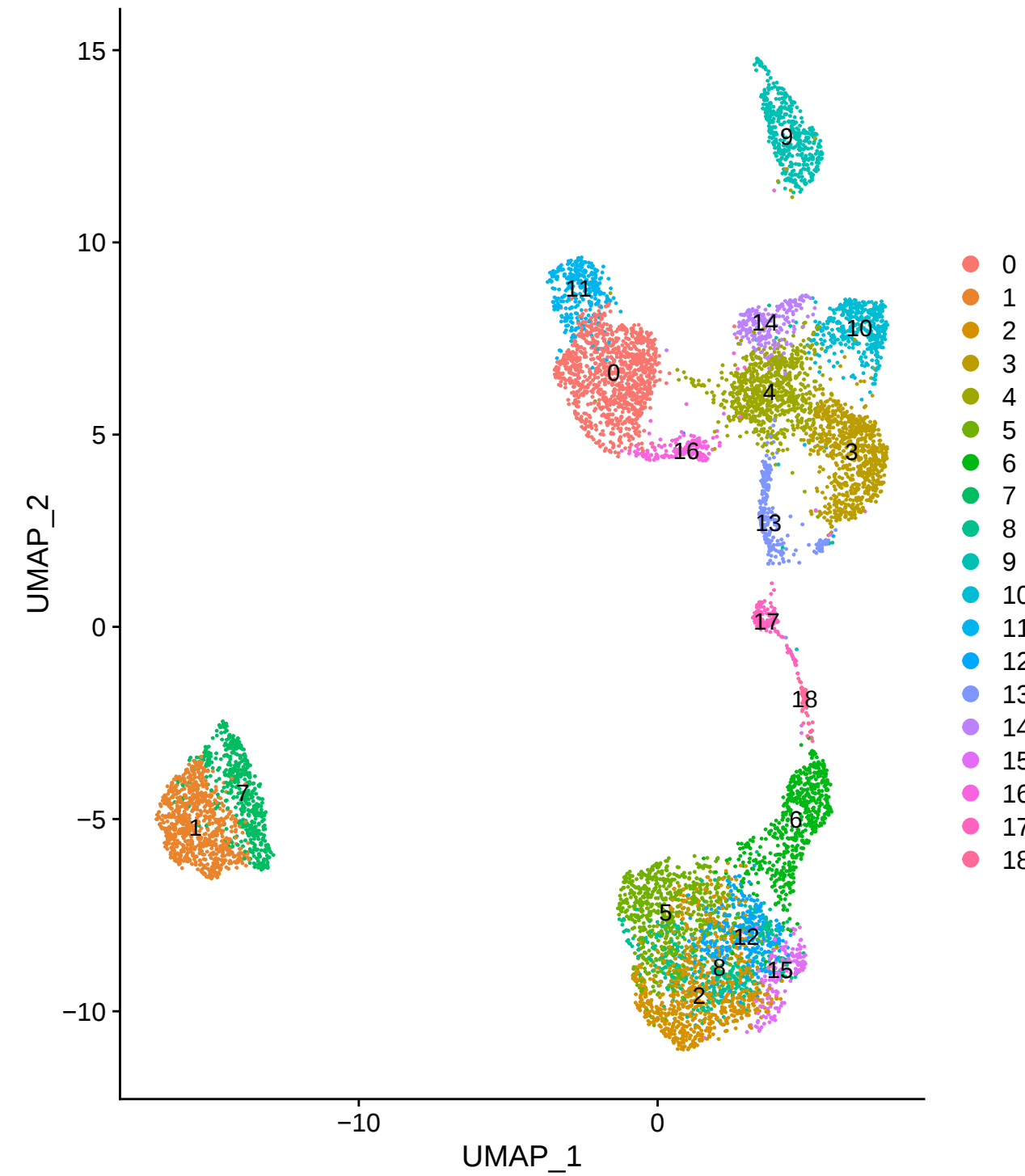
cluster resolution 1.3
