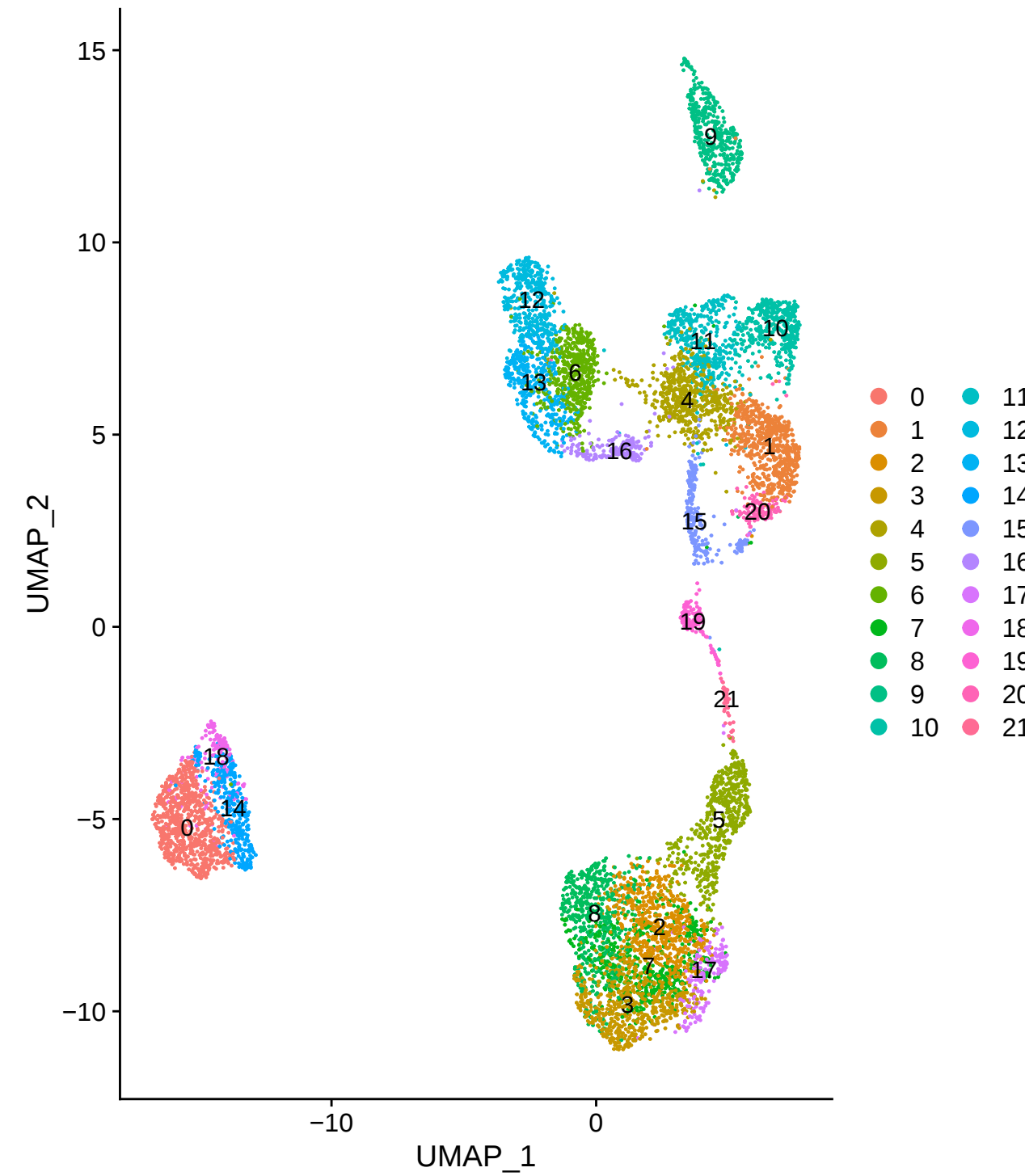
cluster resolution 1.7
