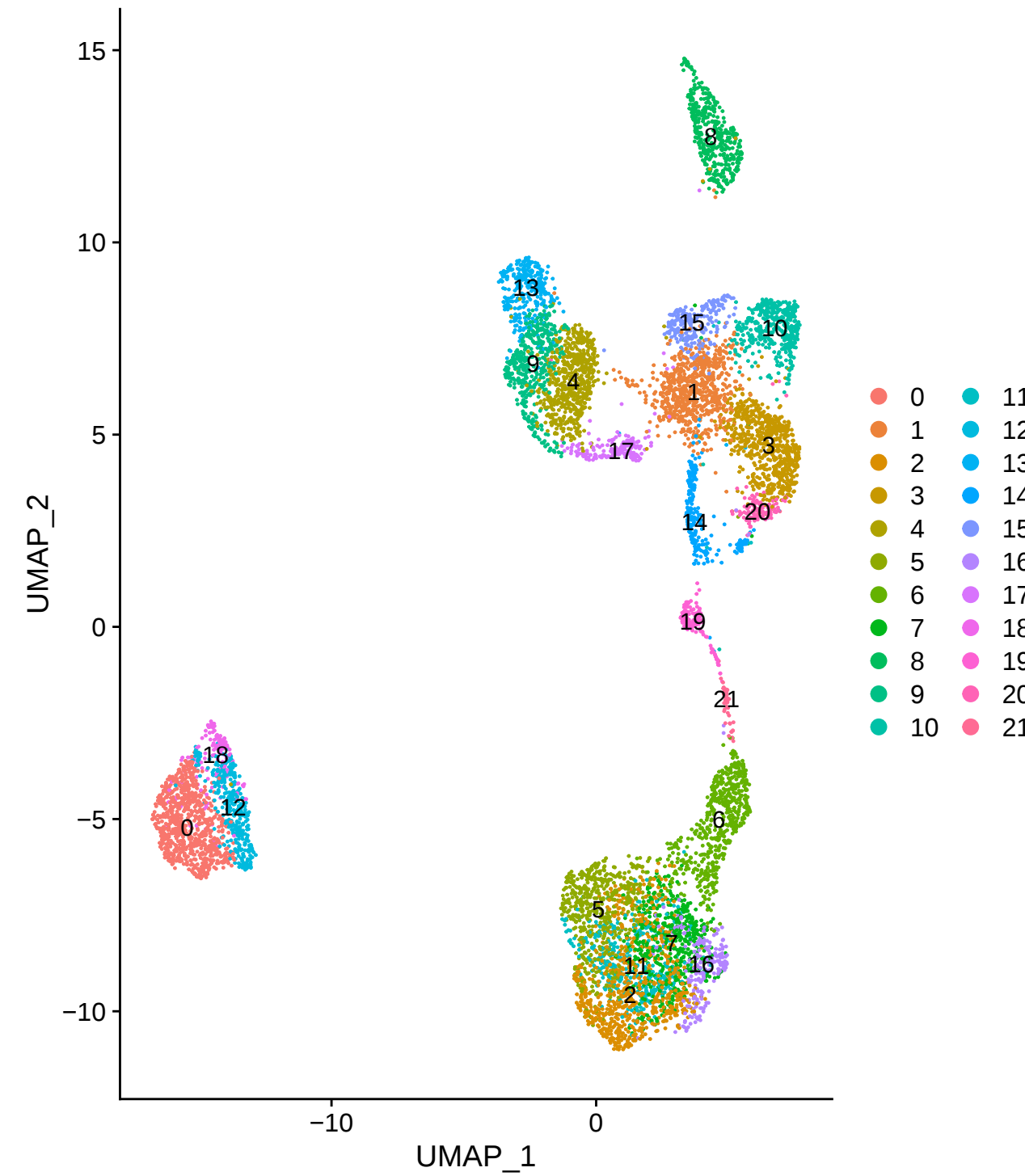
cluster resolution 1.6
