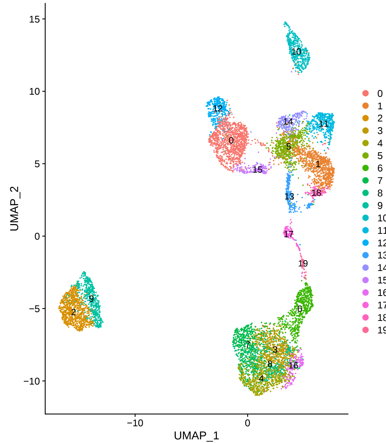
cluster resolution 1.4
