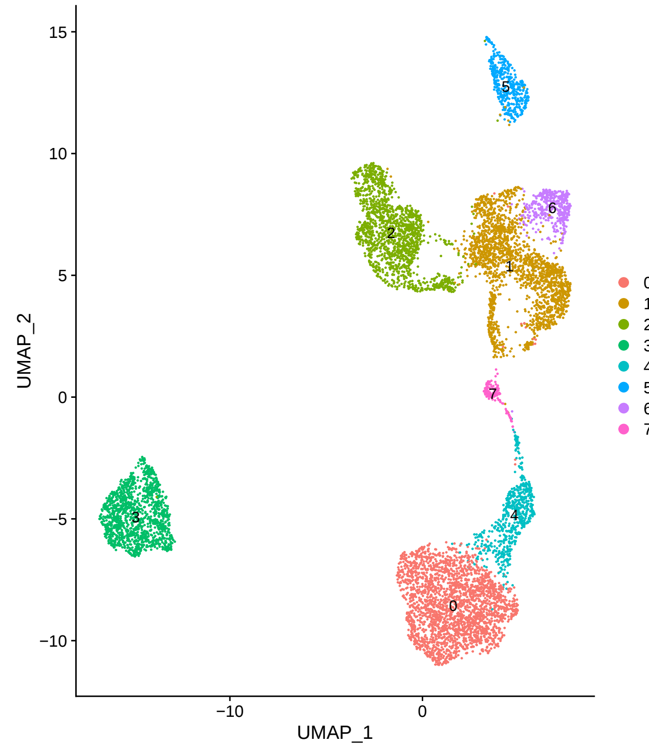
cluster resolution 0.2
