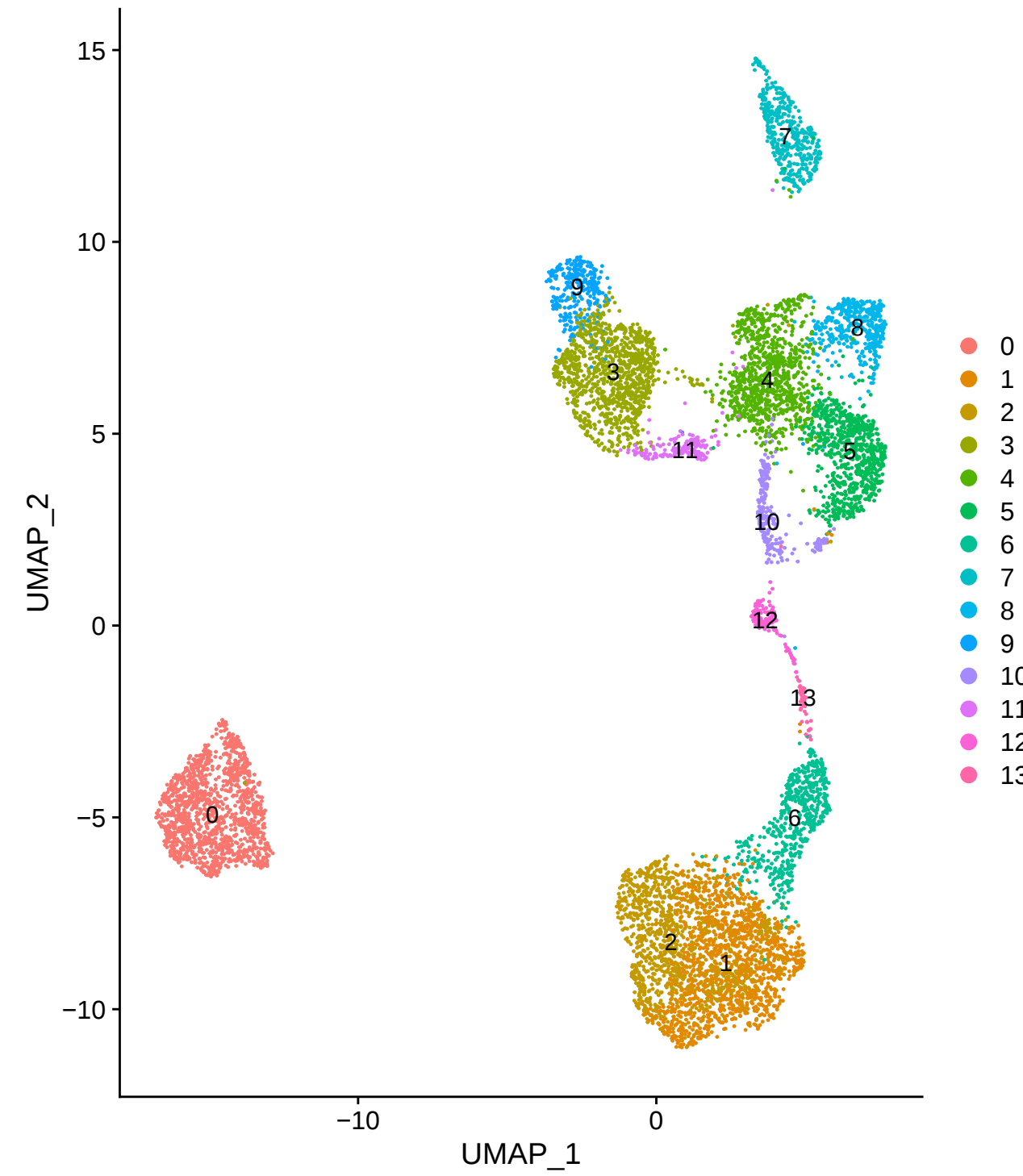
cluster resolution 0.8
