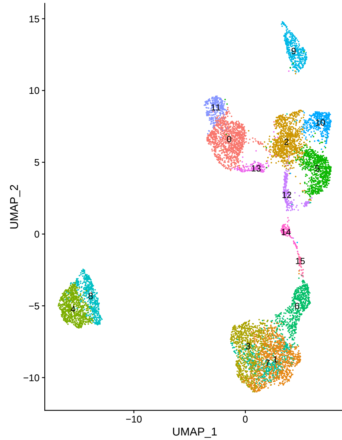
cluster resolution 0.9
