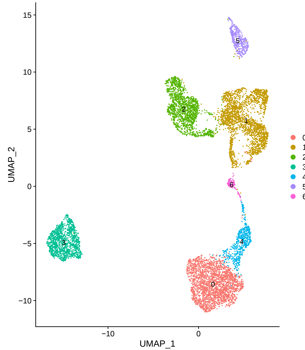
cluster resolution 0.1
