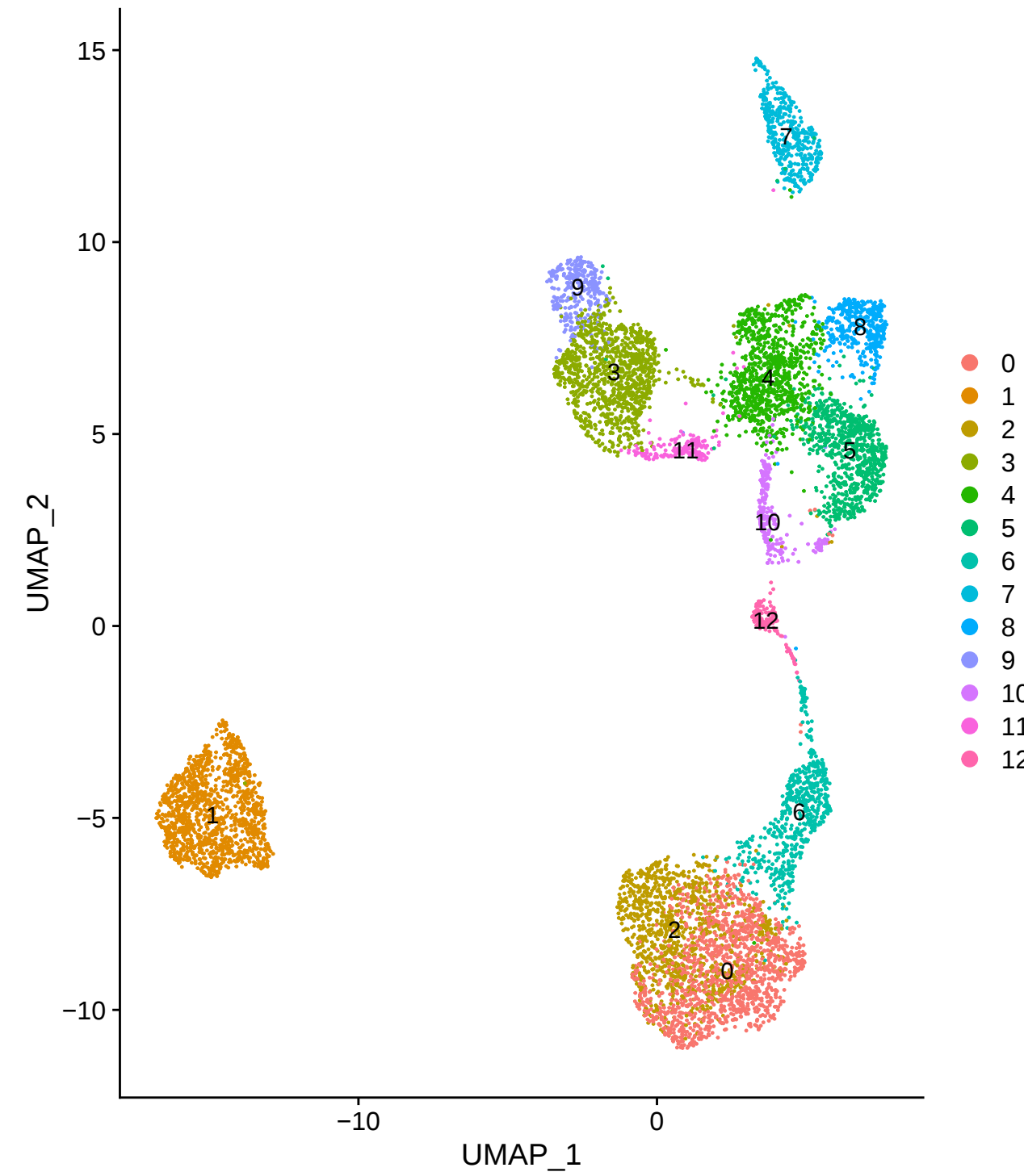
cluster resolution 0.7
