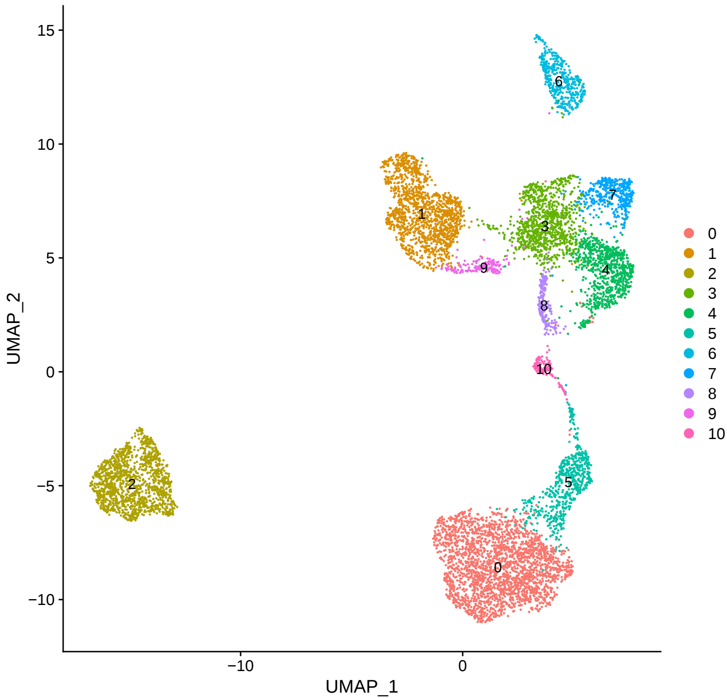
cluster resolution 0.5
