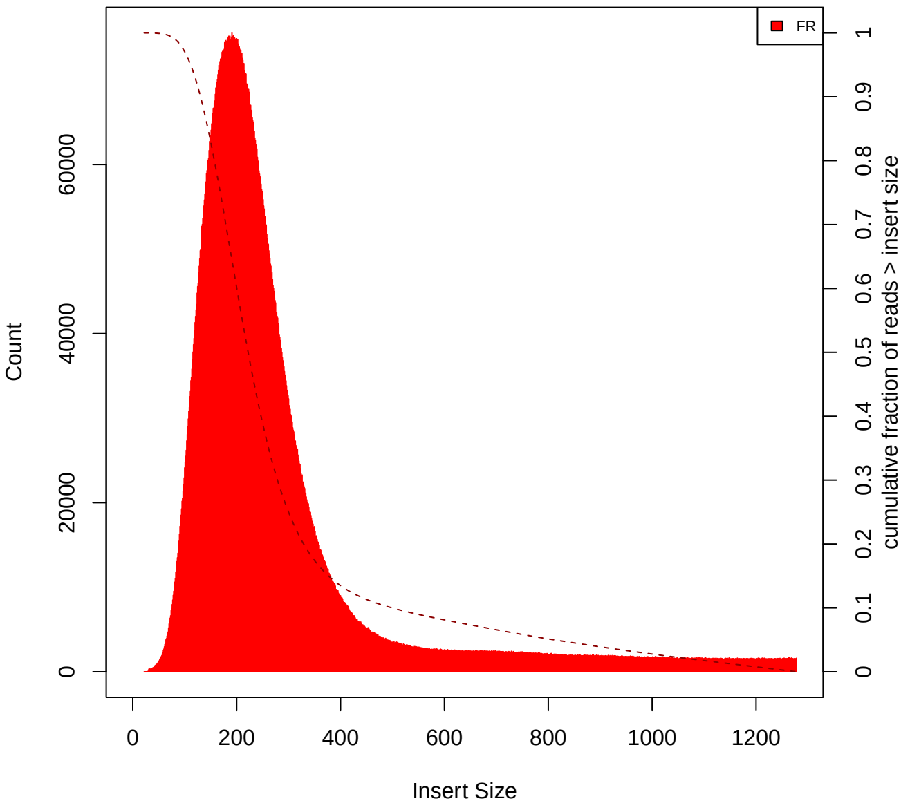
Insert Size Histogram for All_Reads in file GRCh38-DMSO_1.samtools-coordinate.bam
